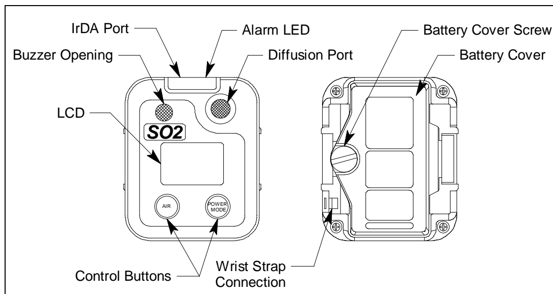
Figure 1: Component Location
