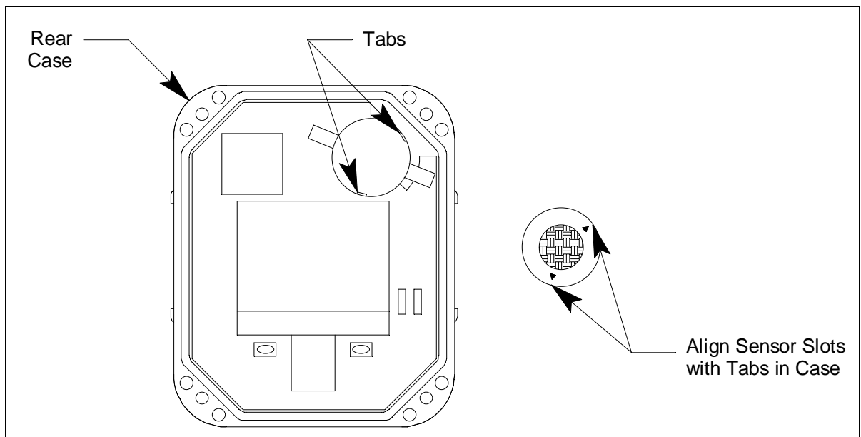
Figure 19: Sensor Location
