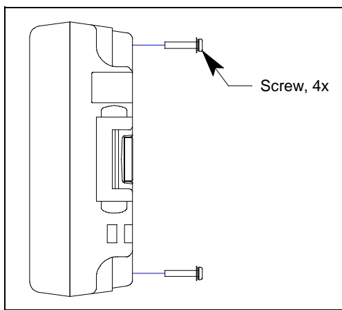
Figure 11: Unscrewing Case Screws
