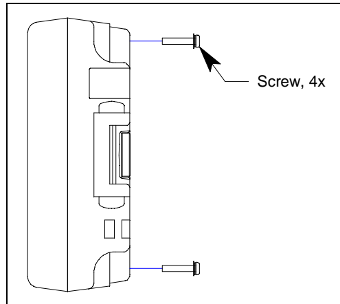
Figure 14: Unscrewing Case
