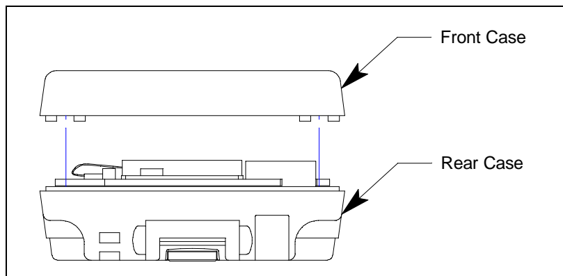
Figure 12: Case Separation
