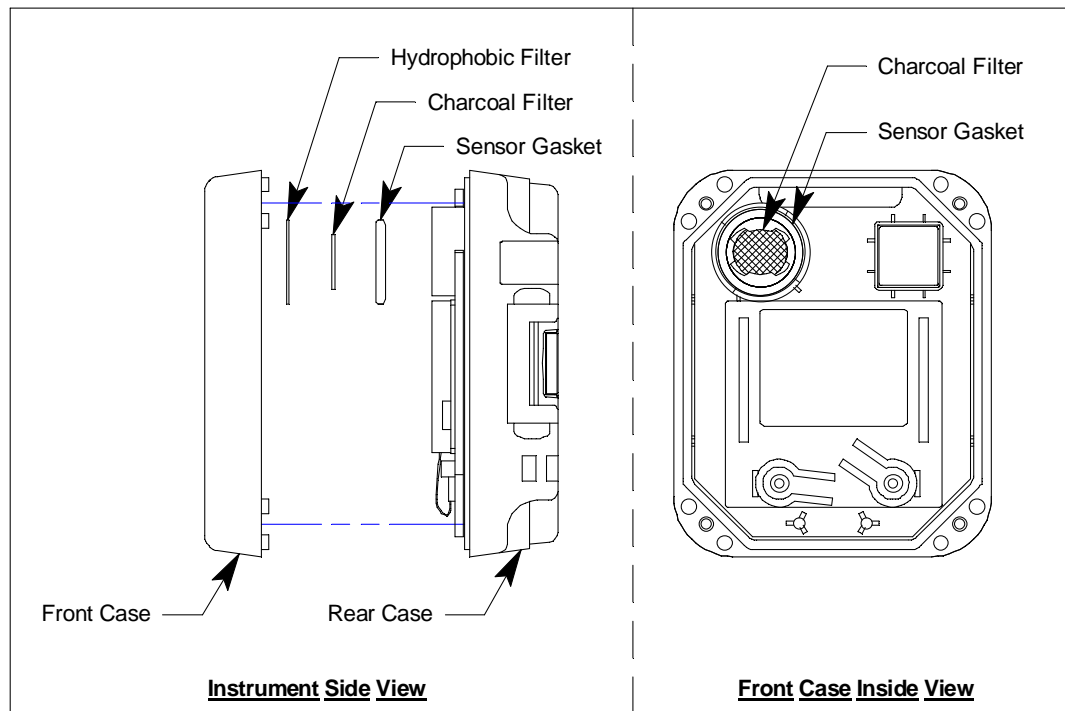
Figure 13: Charcoal Filter Location
