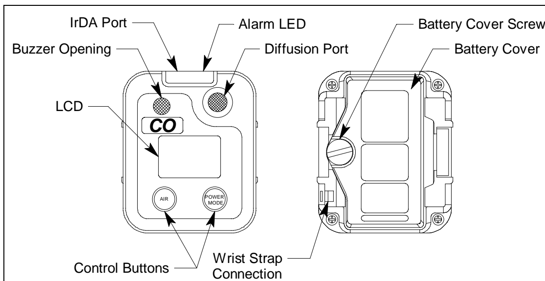
Figure 1: Component Location
