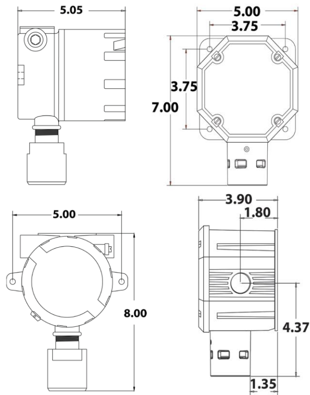
Figure 1 Mounting Dimensions
