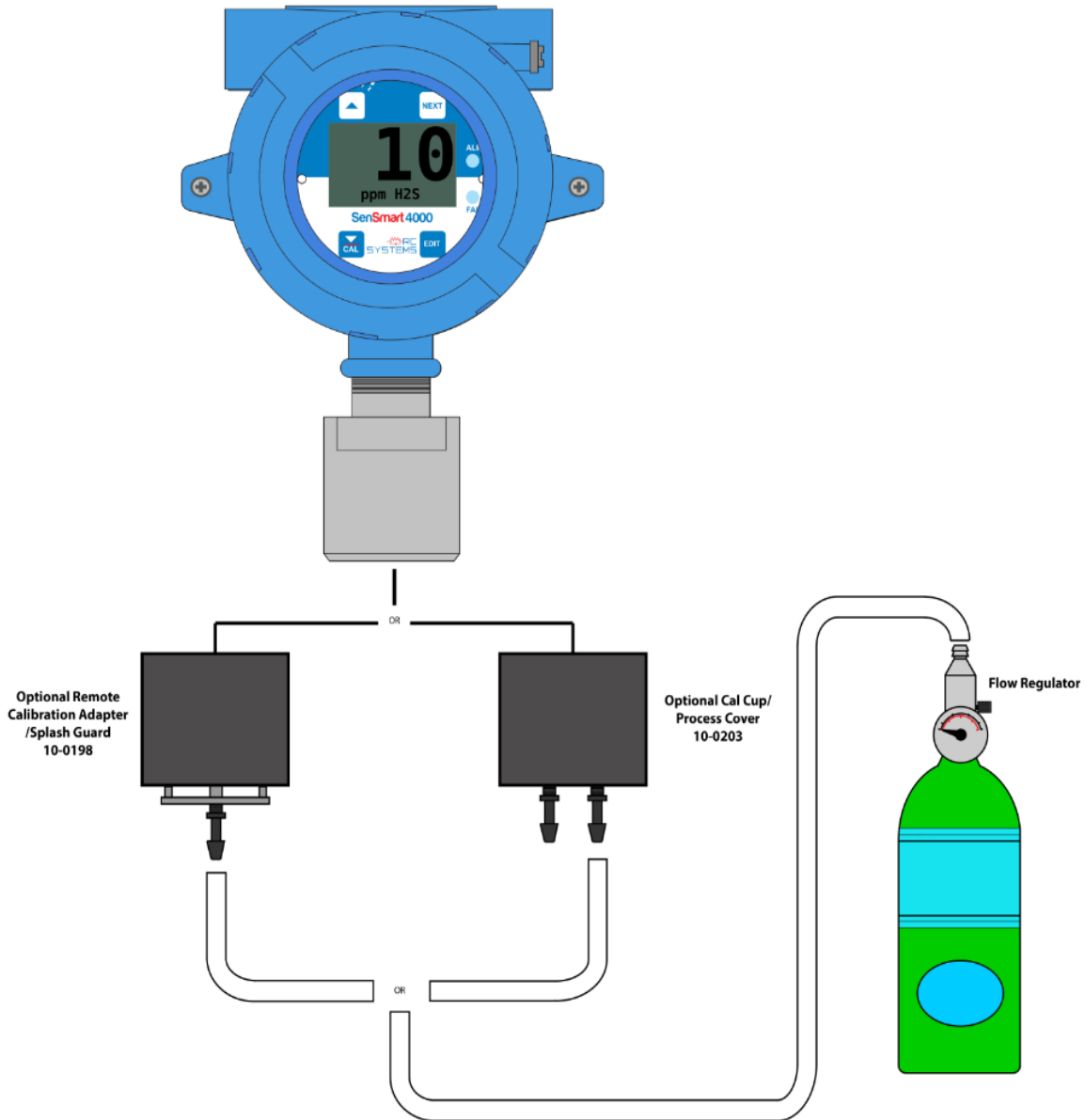
Figure 6 Calibration Diagram
