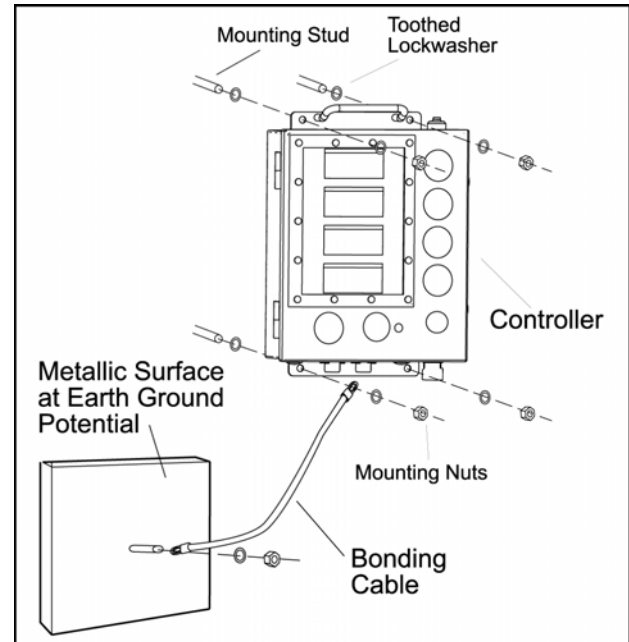
Figure 6. Bonding with Bonding Cable
