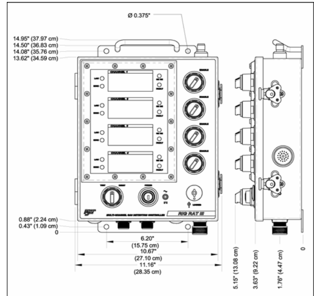
Figure 4. Controller Dimensions
