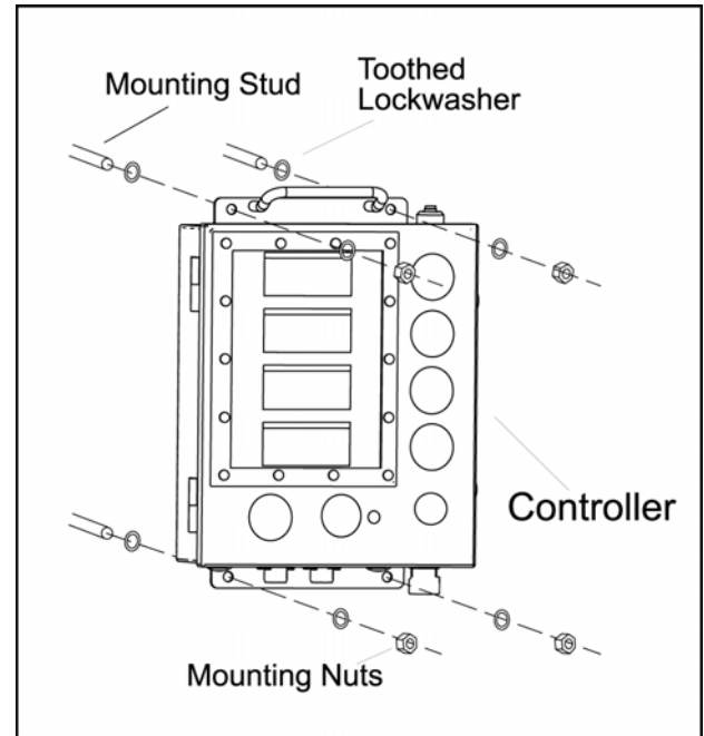
Figure 5. Bonding Controller
