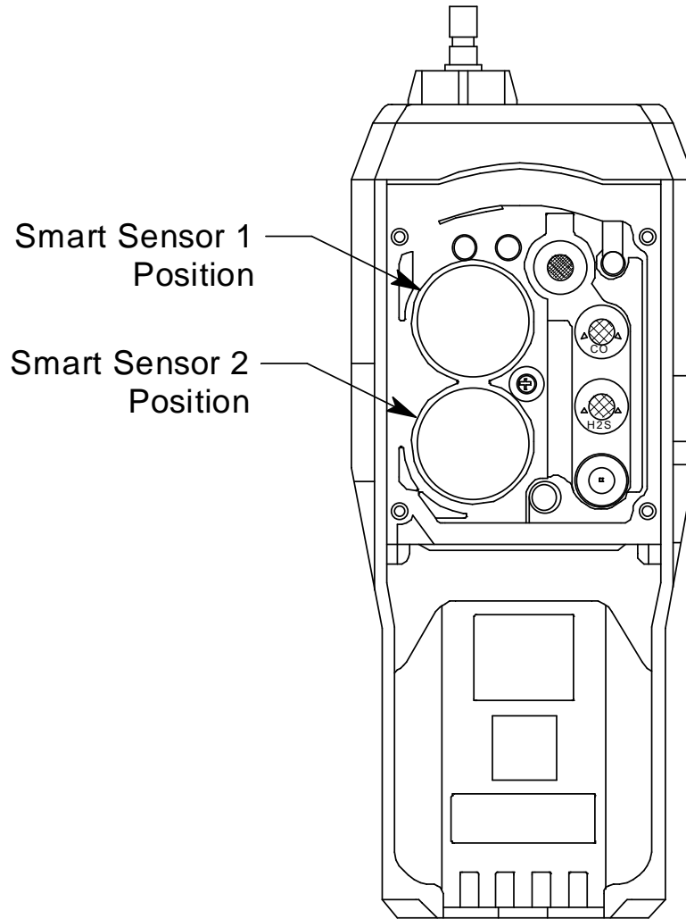
Figure 35: Smart Sensor Positions
