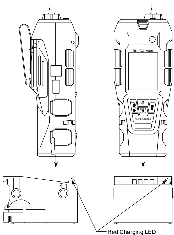
Figure 17: Putting the GX-6000 into the Charging Station
