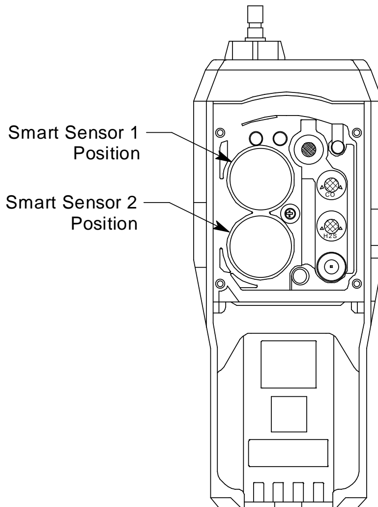
Figure 33: Smart Sensor Positions
