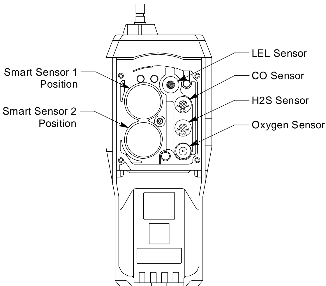
Figure 36: Sensor Location Diagram
