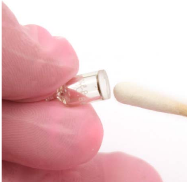
Figure 27: Polishing the Electrode Lamp Window
