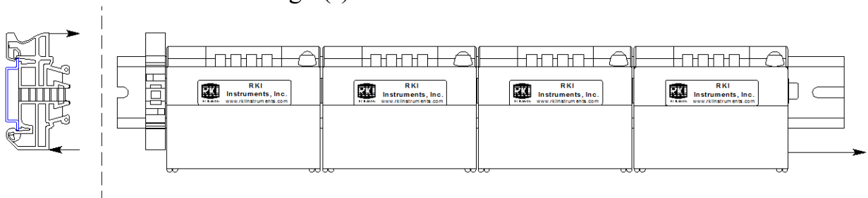
Figure 9: Charger Removal
