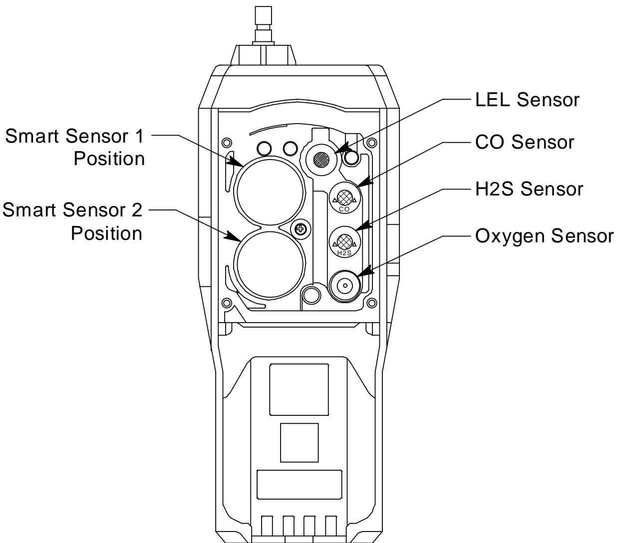
Figure 23: Replacing a Sensor
