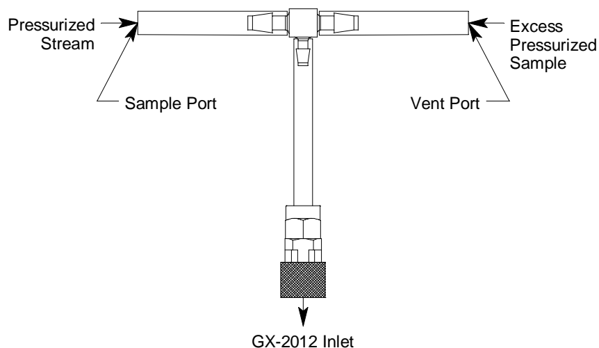
Figure 16: Purge Tee Fitting
