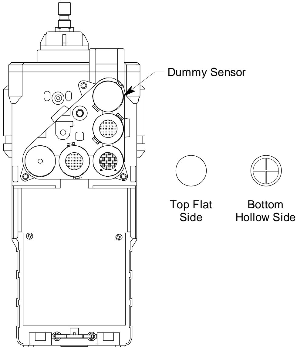
Figure 3: Dummy Sensor
