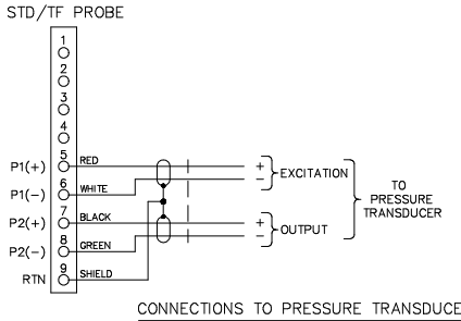
CONNECTIONS TO PRESSURE TRANSDUCER
