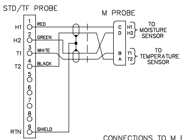
CONNECTIONS TO M PROBE
