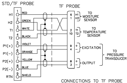
CONNECTIONS TO TF PROBE
