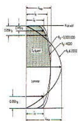
Newtonian velocity profiles
